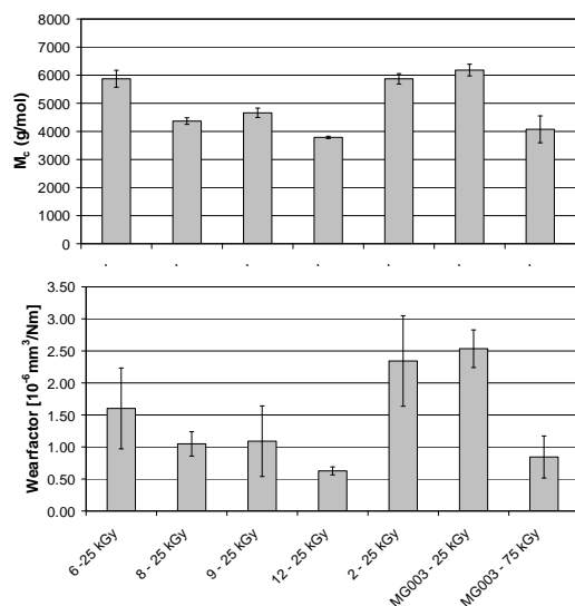
Fig. 2. Molecular Weight between effective crosslinks (top) and wearfactor (bottom) for copolymers with indicated amount of unsaturations (amount of pendant double bonds per 100.000 C-atoms) and indicated gamma radiation dose (kGy).
