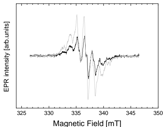
Fig. 3. ESR spectra on octadiene copolymer with 9 vinyl double bonds per 100.000 C-atoms after irradiation with 25 (black) or 75 kGy (grey).
